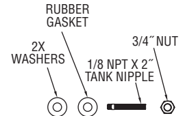
Mounting Hardware
