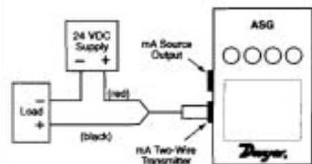
mA Two-Wire XMTR Output
