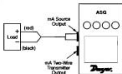
mA Source Output
