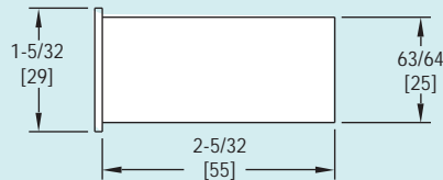
Panel Cutout 2.36" x 1" (60 x 26 mm)
