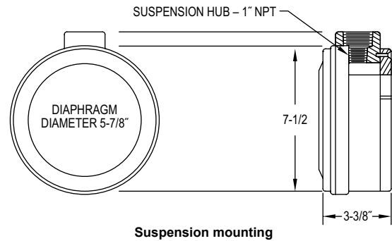
Suspension mounting
