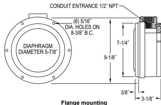
Flange mounting
